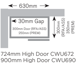
Corner Wall Unit
