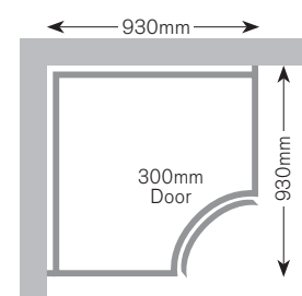
Full Height Door COB991PCF
