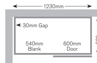
Full Height Door CB126F Drawer Line CB126D
