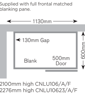
Corner Larder Unit
