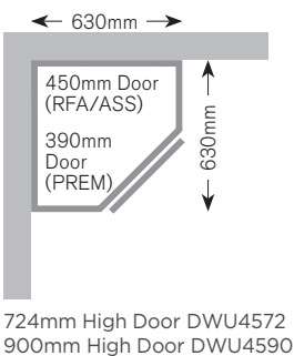
Diagonal Corner Wall Unit
