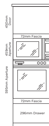
Single Oven & Microwave/ Compact Oven Housing (1A) †
