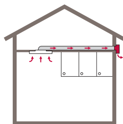
DDMEXT3 with ceiling
