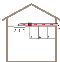
DDMEXT25 for ceiling
